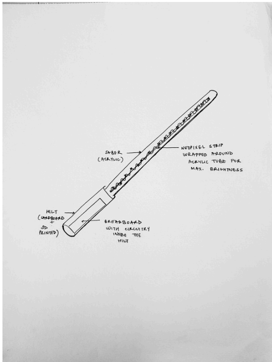
More sketches & component finalisation
